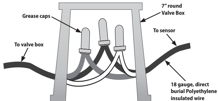
Figure 6 Wiring Box Connections
